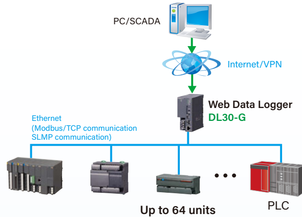
The DL30-G can be expanded by connecting to remote I/O and SLMP-compatible devices.
