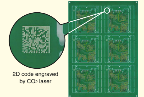
PCB for the high-mix, low-volume production
