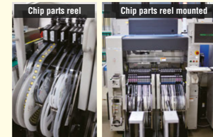
High-mix, low-volume production-compatible multiple in-line chip mounters
