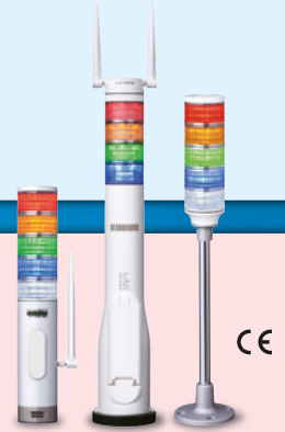
(Left to right) W90 x H352 x D60 mm (IT60SW5) W98 x H667.4 x D98 mm (IT60W1) W94 x H490.5 x D94 mm (IT60SA3) CE
