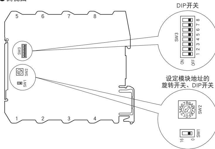
● 侧视图
