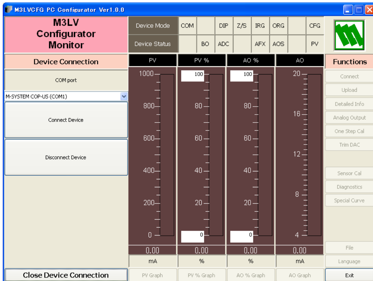
Figure 2. Device Connection
