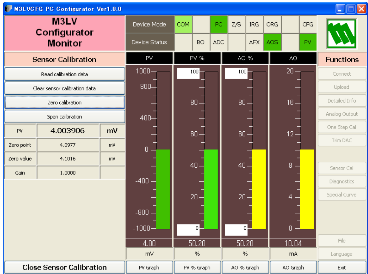
Figure 9. Sensor Calibration
