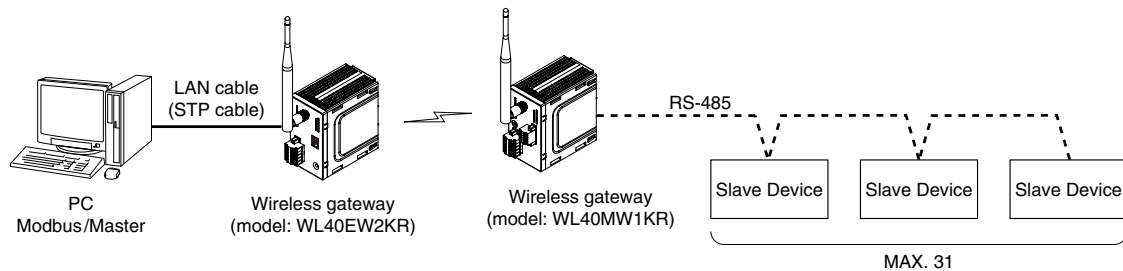
Figure 1.1 System configuration example
