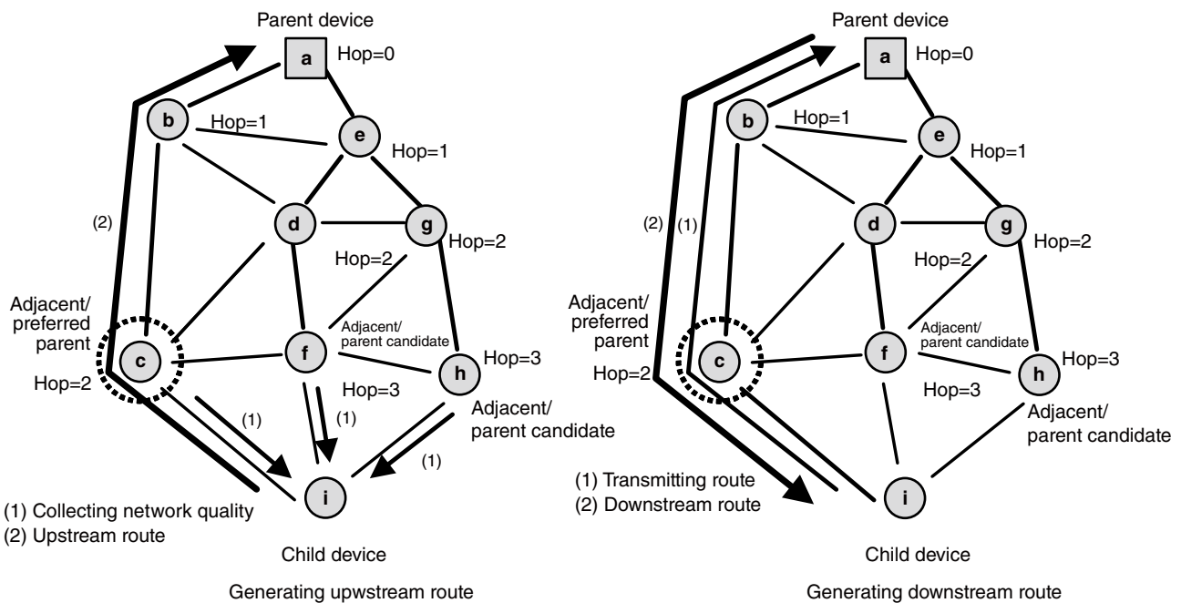
Figure 3.1 Wireless network
