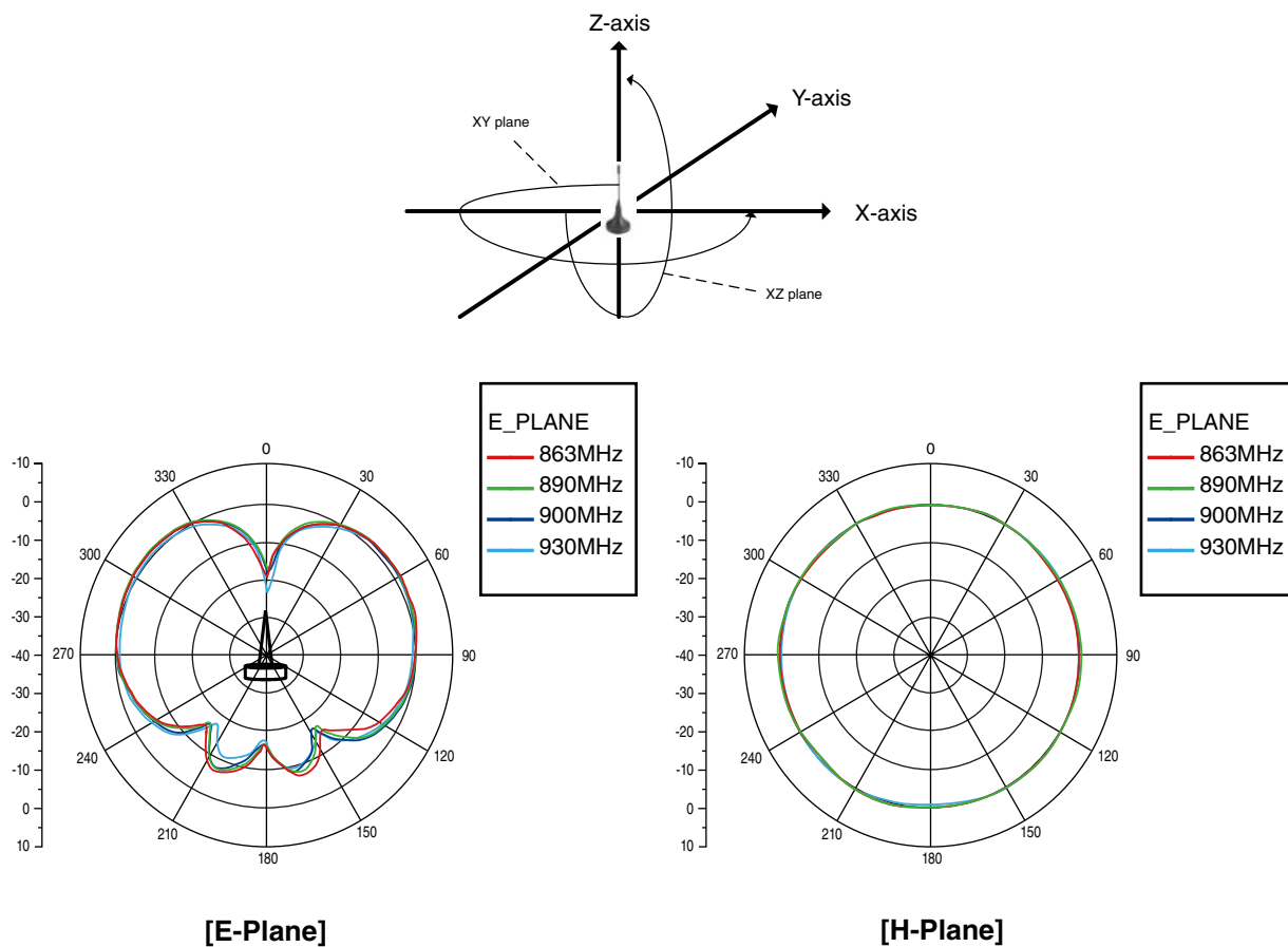
Figure 9.3 Directionality of rooftop antenna for WL40KR series <reference>
