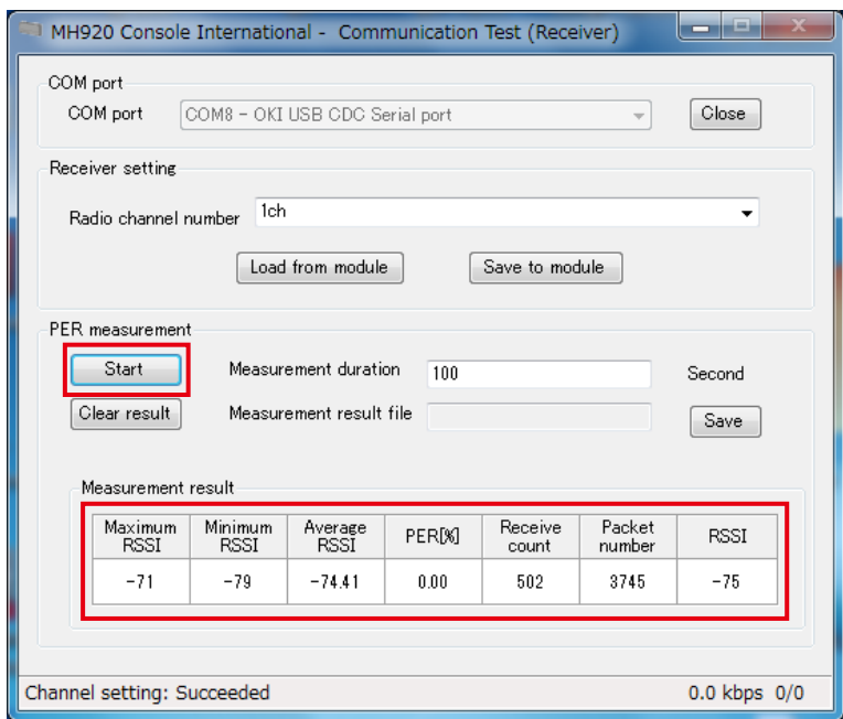
Figure 6.35 Measurement result
