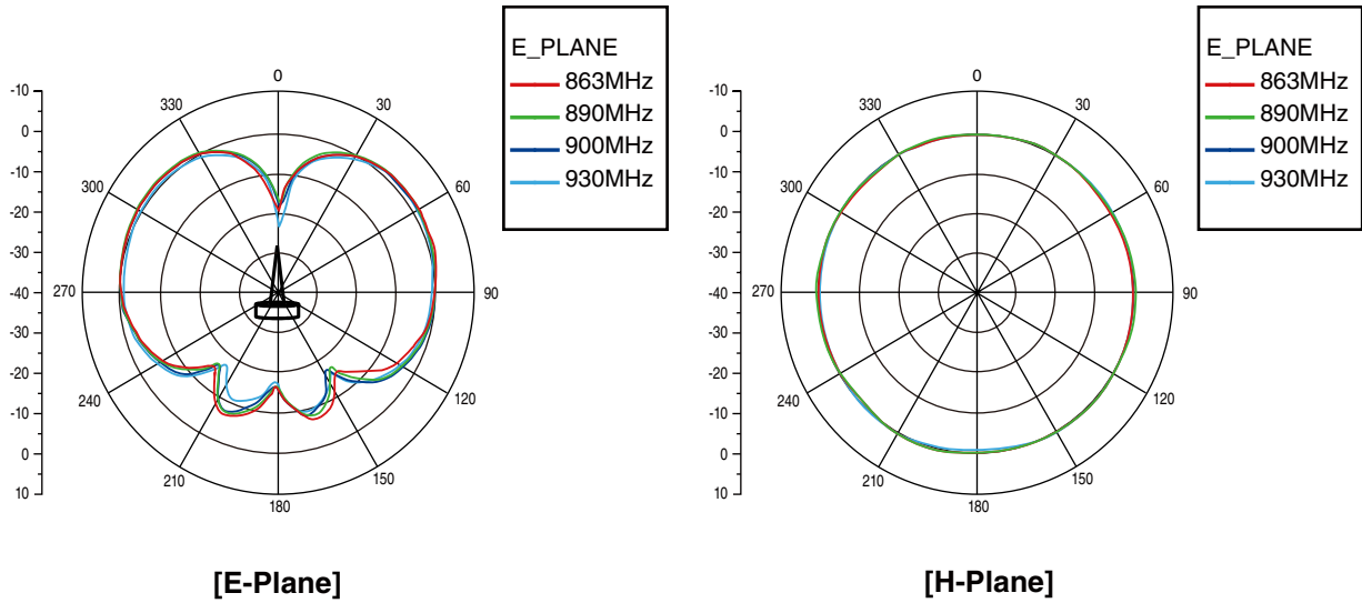
Figure 9.3 Directionality of rooftop antenna for WL40KR series <reference>
