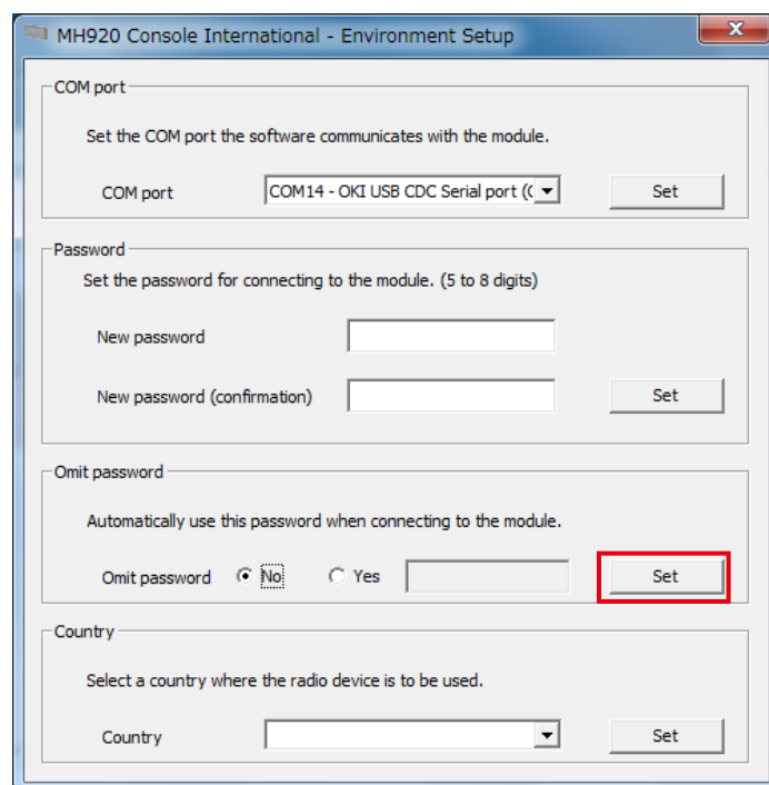
Figure 5.25 “Omit password” setting
