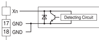
■ 2-Wire Sensor
