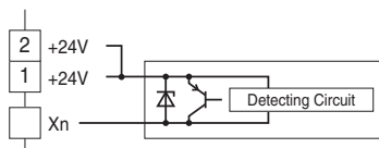
■ 2-Wire Sensor
