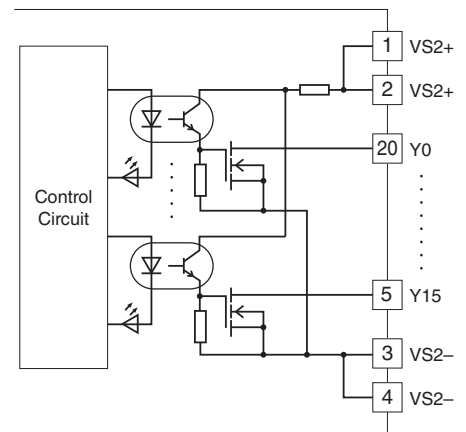
■ Output Circuit
