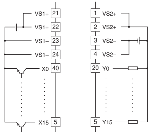
■ Input Connection Example
