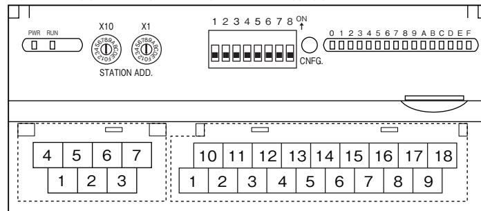
Network, Power Supply Terminals
