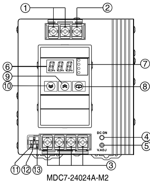
MDC7-24024A-M2
